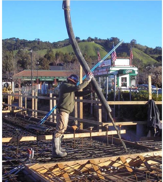
Beginning concrete pour on Second Level (at the Children's Area near the Seaborg Garden)
